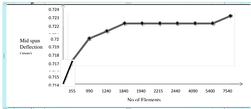
Fig 4: Results of the convergence study
