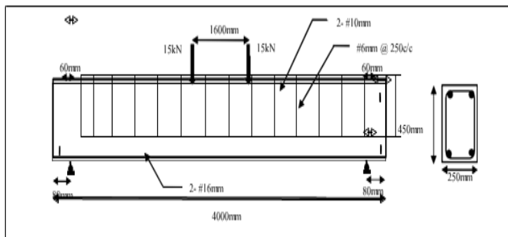
Fig 1: Beam considered for the study
